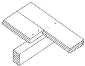
2 nails a joist over 85 mm cover
