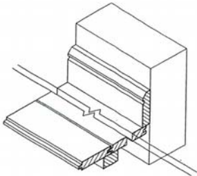
10 mm min. gaps at each wall
